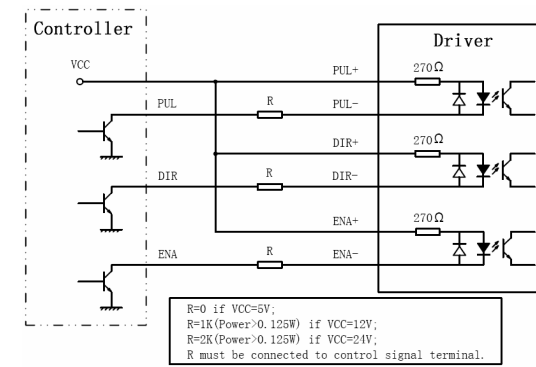
Figure 2: Connections to open-collector signal (common-anode)
