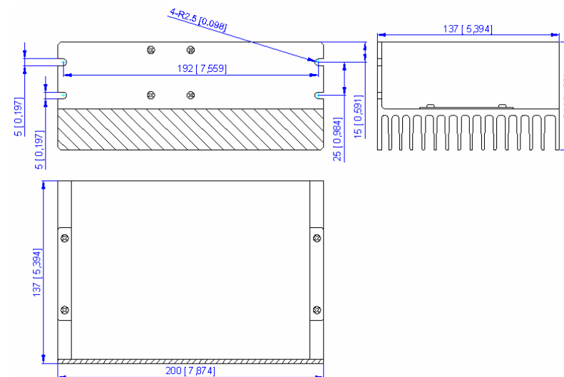
Figure 1: Mechanical specifications
